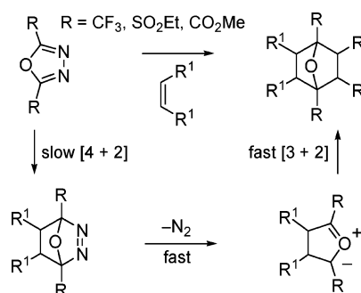
Figure 1. 1,3,4-Oxadiazole cycloaddition cascade.
